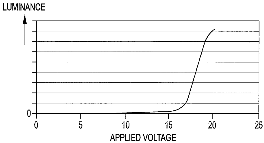
LUMINANCE vs. APPLIED VOLTAGE FOR 17" EL
