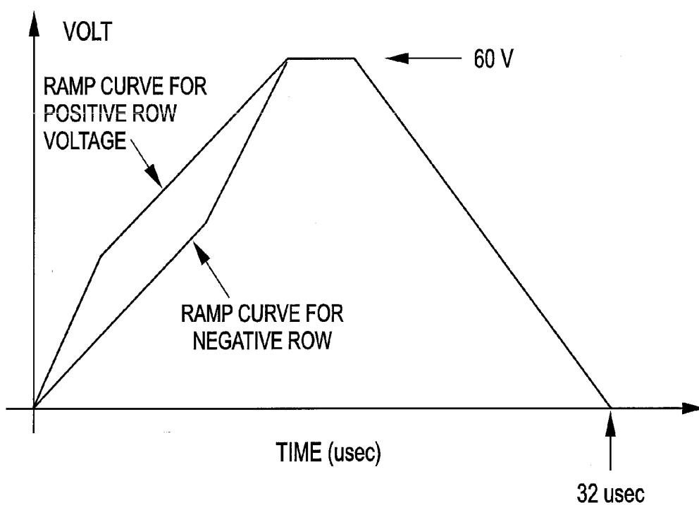
STEPWISE LINEAR APPROXIMATION OF GAMMA CORRECTION CURVE
