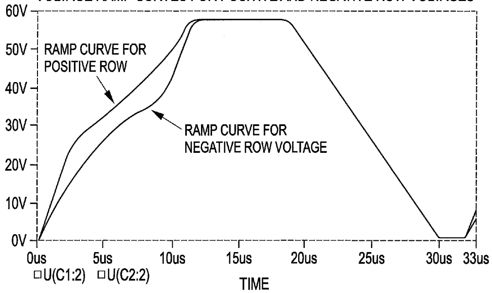
VOLTAGE RAMP CURVES FOR POSITIVE AND NEGATIVE ROW VOLTAGES
